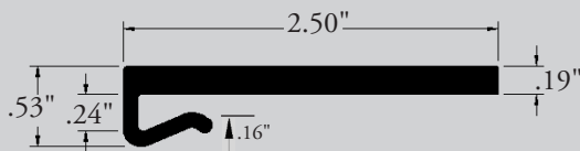
PS-546 2.5\" J-LEG
