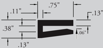
PS-566 3/4\" BAR-CLIP
