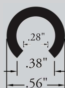
PS-551 3/8" FULL ROUND SNAP-ON
