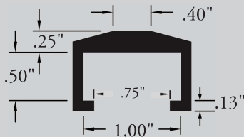
PS-528 1" x 1" DRIVE BAR CAP
