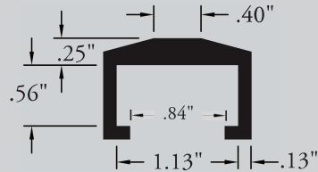
PS-534 1-3/16" x 1-3/16" DRIVE BAR CAP
