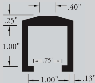
PS-528 1" x 1" DRIVE BAR CAP
