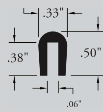
PS-568 BAR CLIP-ON
