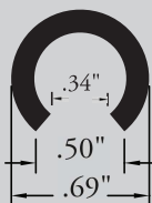
PS-550 1/2" FULL ROUND SNAP-ON
