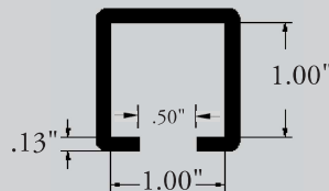
PS-524 1" x 1" GUIDE RAIL SNAP-ON
