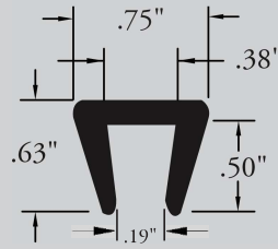
PS-562 BAR CLIP-ON
