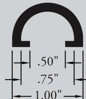
PS-552 3/4" HALF ROUND SNAP-ON
