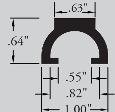
PS-553 3/4" FLAT TOP SNAP-ON
