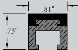
PS-502 C-RAIL ASSY.
