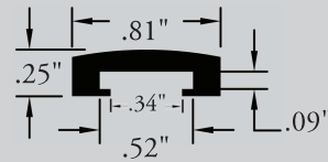
PS-503 C-RAIL COVER
