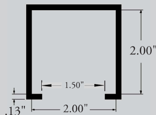
PS-532 2" x 2" GUIDE RAIL SNAP-ON
