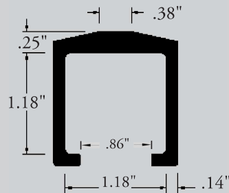
PS-534 1-3/16" x 1-3/16" DRIVE BAR CAP
