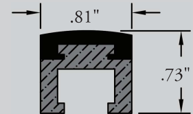
PS-504 C-RAIL ASSY.
