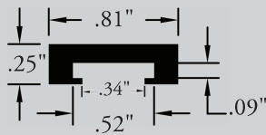
PS-501 C-RAIL COVER
